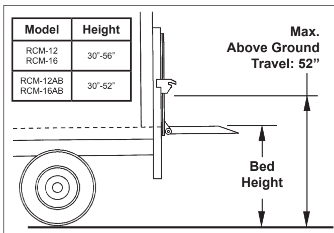
Mounting Requirement Dimensions
